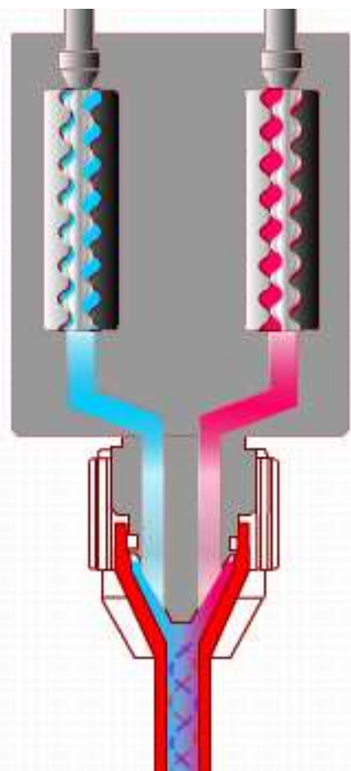
Screw Metering Arrangement
